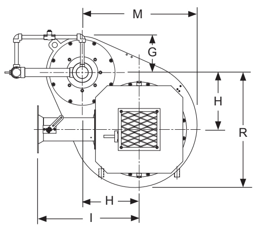
45° Slant Position End View - Slant Right Shown (FGR & Gas inlets can be on left or right side) Slant left available
